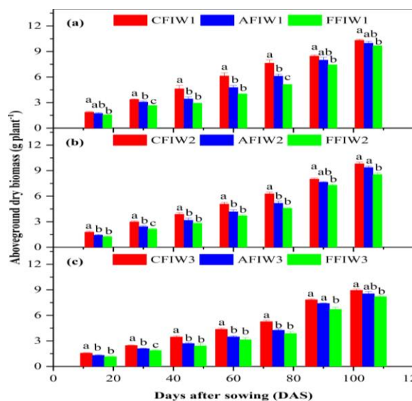
Figure 6. Above-ground dry biomass under different treatments at W1 (a), W2 (b), and W3 (c) irrigation levels
