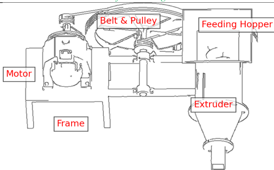
Figure 2. Sketch of logs making machine Table 1. Specifications of log-making machine
