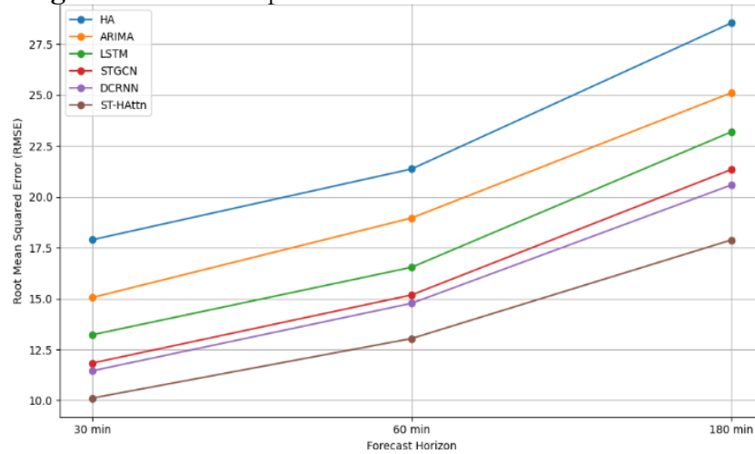
Figure 3. RMSE vs Forecast Horizon For Different Models
