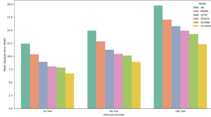
Figure 2. MAE Comparison of models Across Forecast Horizon
