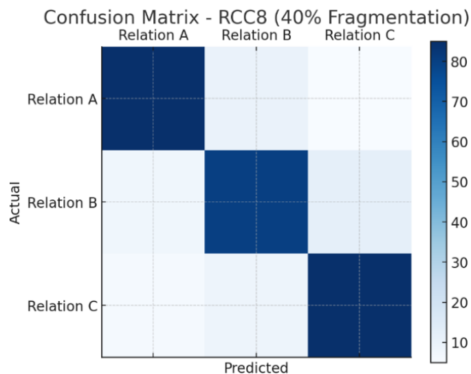
Figure 2. Confusion Matrix – RCC8 Model at 40% Fragmentation
