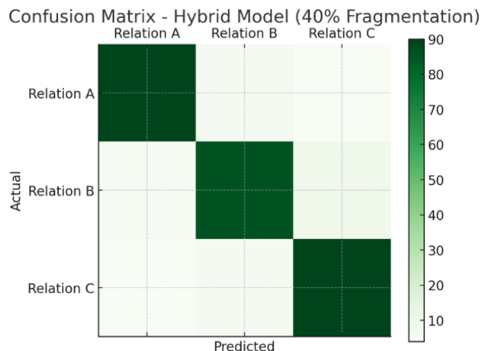
Figure 3. Confusion Matrix – Hybrid Model at 40% Fragmentation
