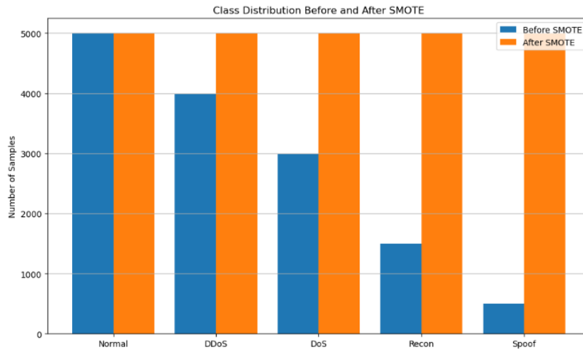
Figure 1. Class distribution before and after SMOTE
