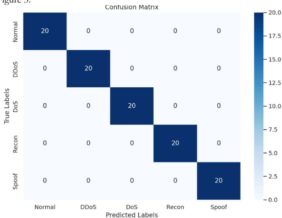
Figure 3 presents the confusion matrix for the best-performing configuration (RF with SMOTE + PCA). The diagonal dominance indicates a high number of correct predictions for all classes, including previously underrepresented ones. Misclassifications are minimal, highlighting the model's robust generalization ability across diverse attack types.
