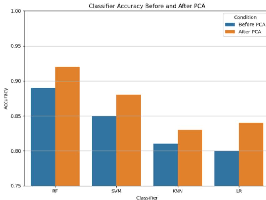
Figure 2. Classifier Accuracy before and after PCA
